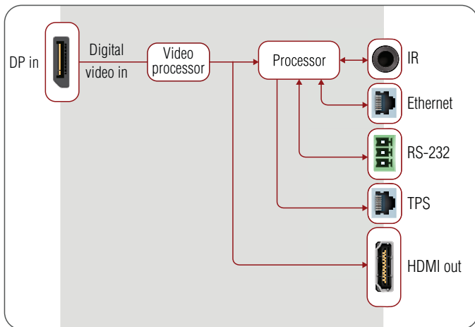
Port diagram
