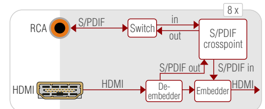
MX-HDMI-3D-IB-S
